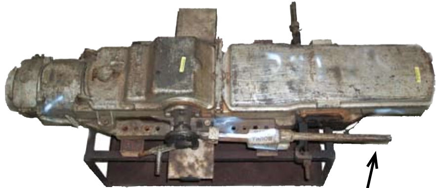
A used switch machine arrives at our facility....
