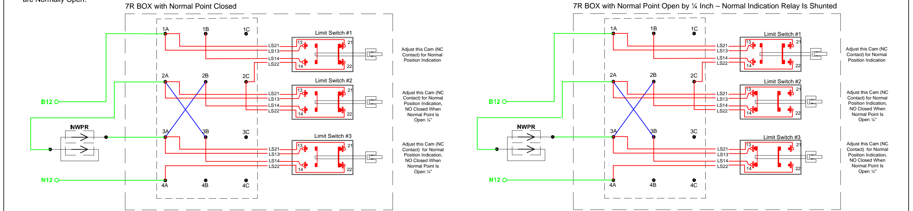
Figure A-1. 7R Switch Circuit Controller Circuit 48950-310-00
