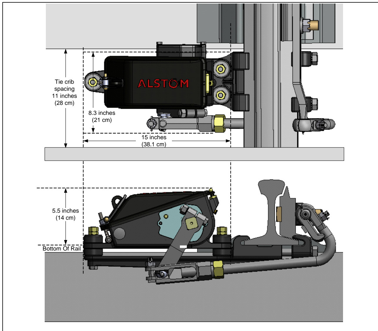
Figure 1–2. Model 7R Switch Circuit Controller Dimensions
