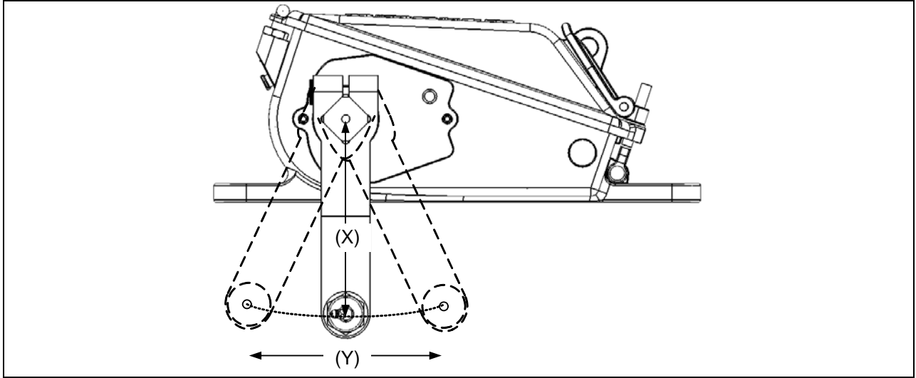
Figure 1-5. Controller Crank Arm Throw
