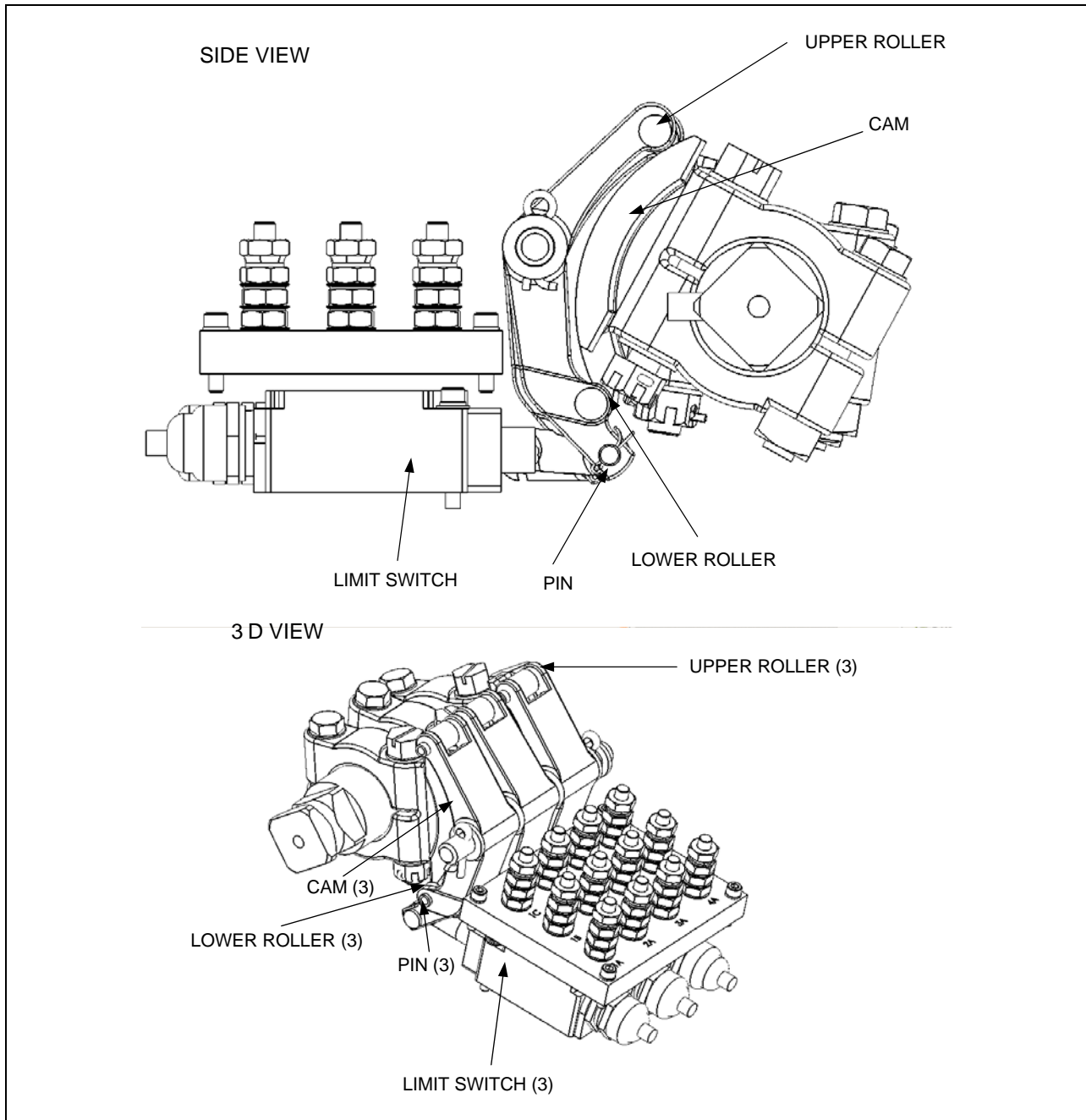
Figure 1–1. Model 7R Push Pull Mechanism
