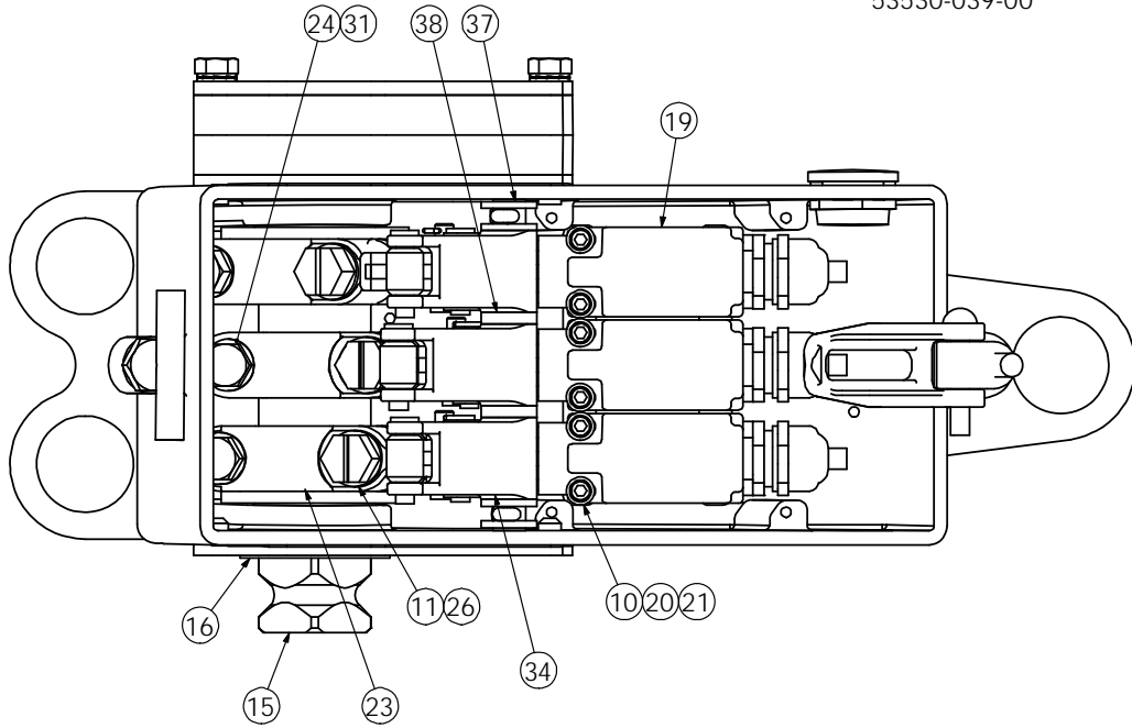
VIEW SHOWN WITH COVER COMPLETE (REF.2) AND CRANK COMPLETE (REF.18) REMOVED
