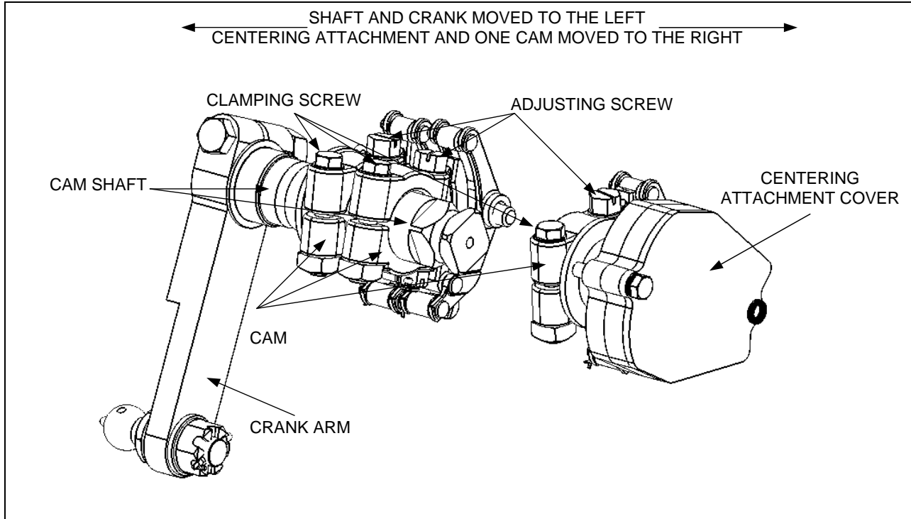
Figure 1-4. Cams Detail
