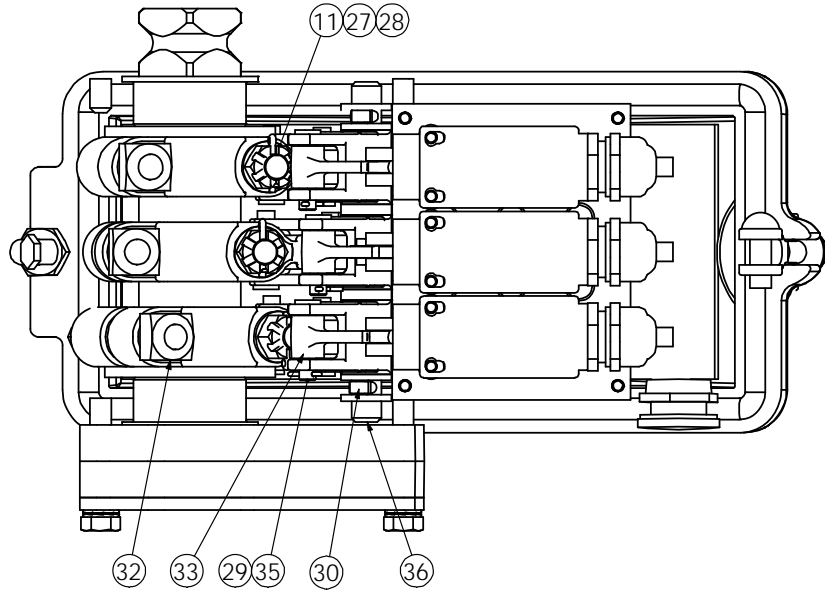
BOTTOM VIEW SHOWN WITH CASE (REF.1) AND CRANK COMPLETE (REF.18) REMOVED
