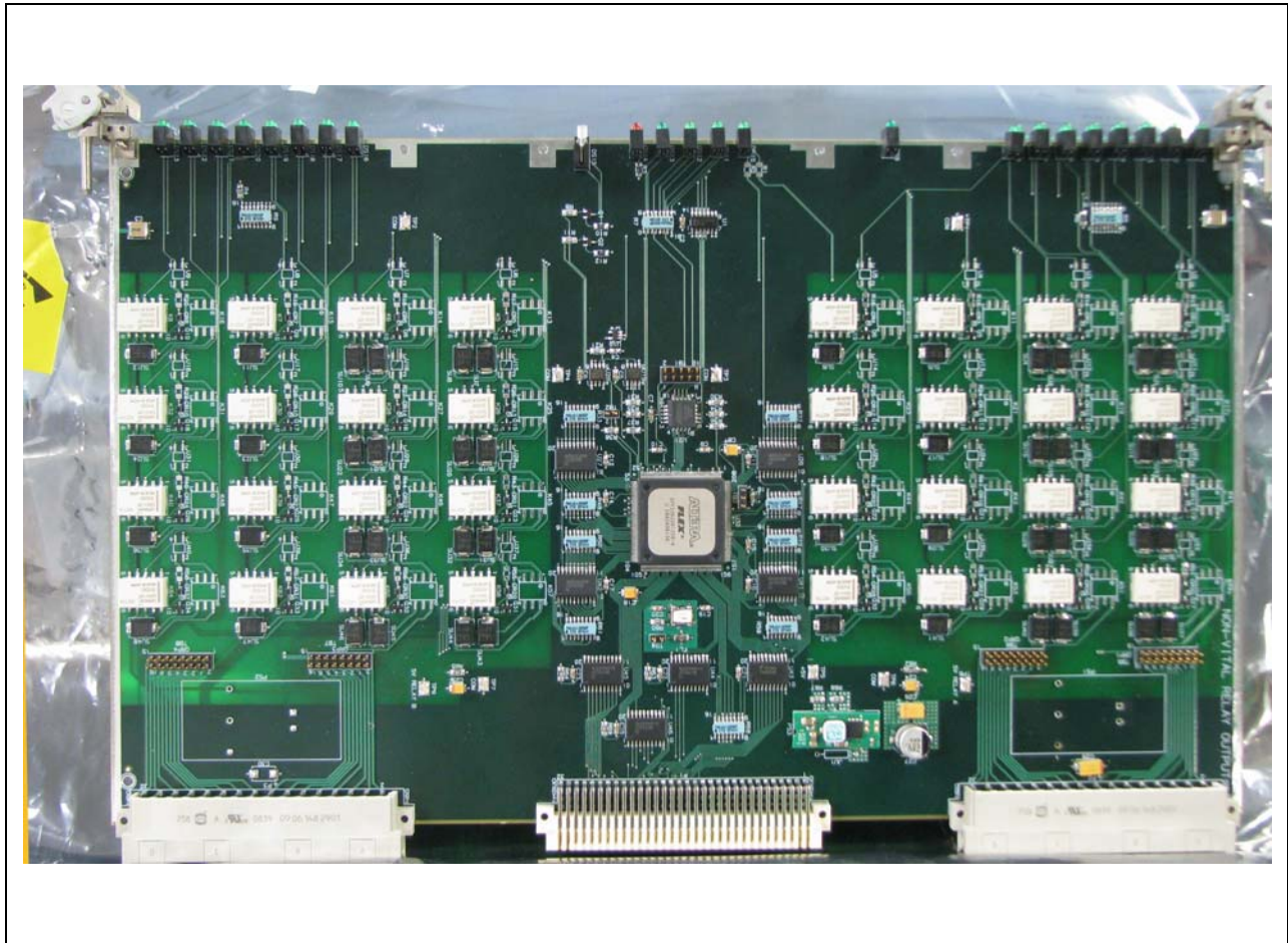
Figure 5–2. NVO Board
